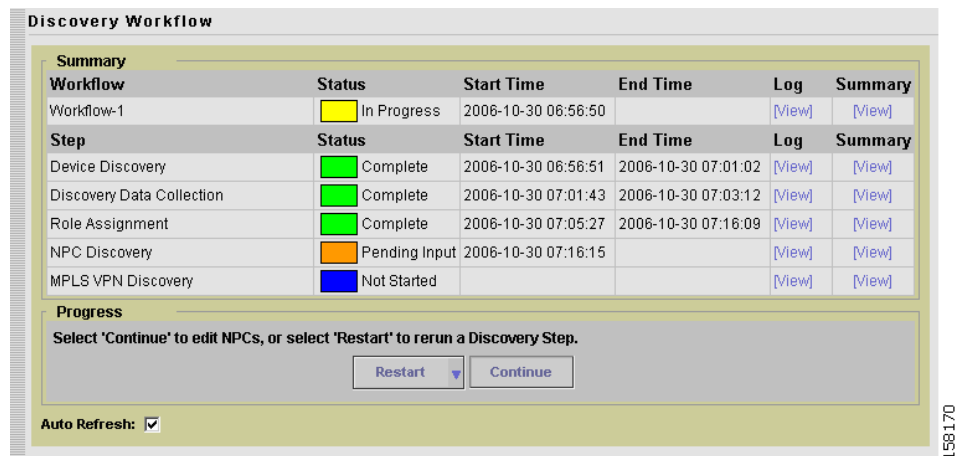
Figure 4-35 Discovery Workflow Window with MPLS VPN Discovery Pending Input
