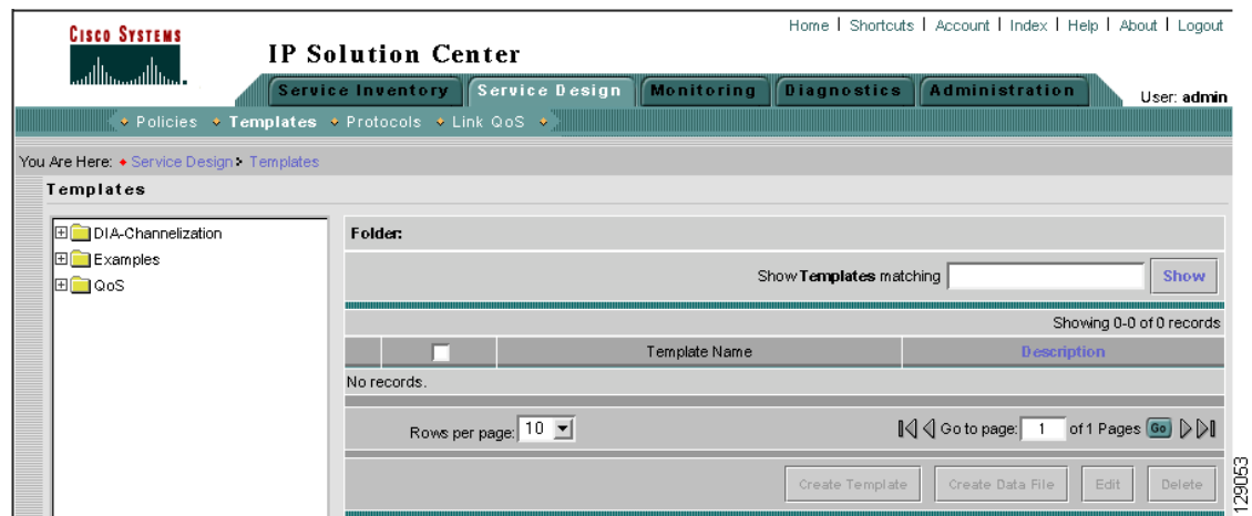
Figure 6-2 Templates
