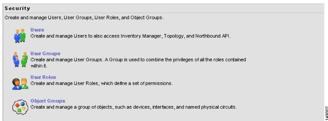
Figure 1-17 Security Selections
