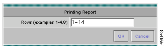
Figure 7-61 Print Report
