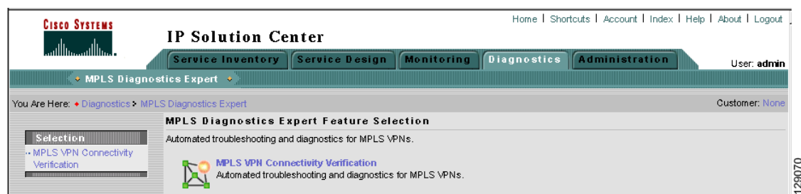
Figure 1-15 Diagnostics Selections
