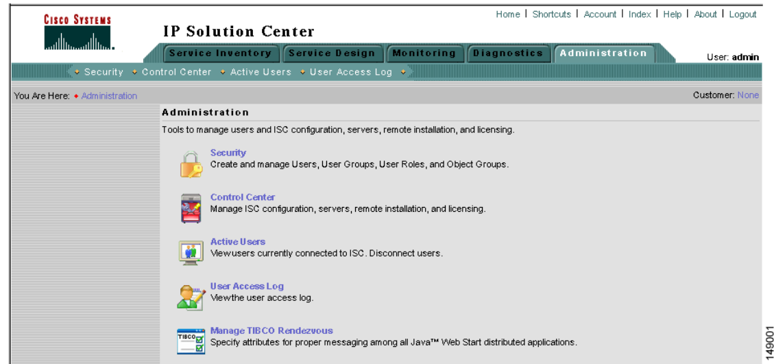
Figure 1-16 Administration Selections
