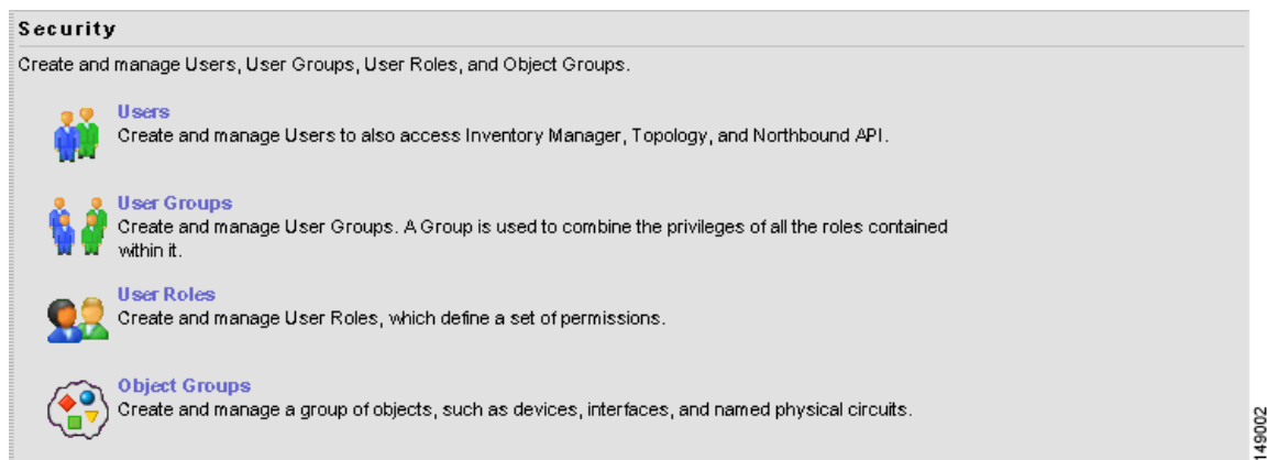
Figure 1-17 Security Selections
