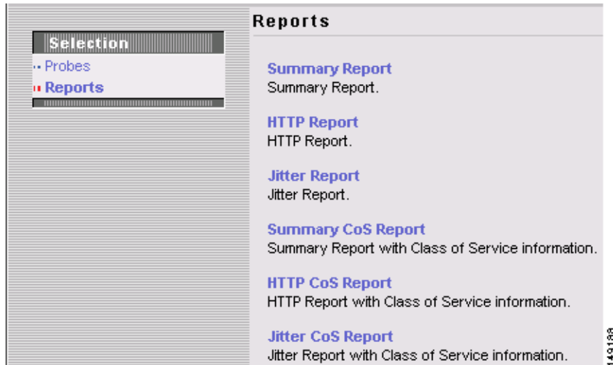
Figure 7-54 SLA Reports
