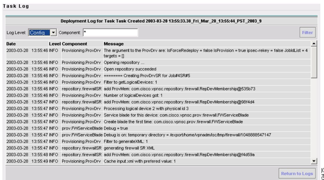
Figure 7-10 Task Log
