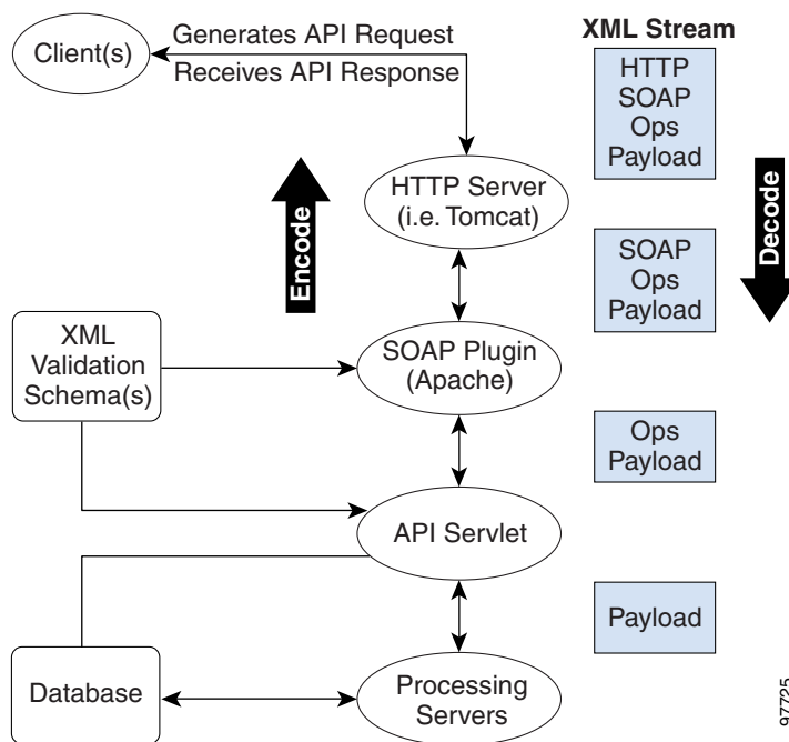
Figure 1-1 API Components
