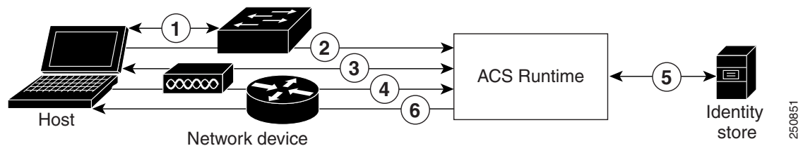
Figure A-2 RADIUS-Based Flow Without EAP Authentication
