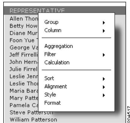
Figure 13-4 Context Menu for Column Data in Interactive Viewer
