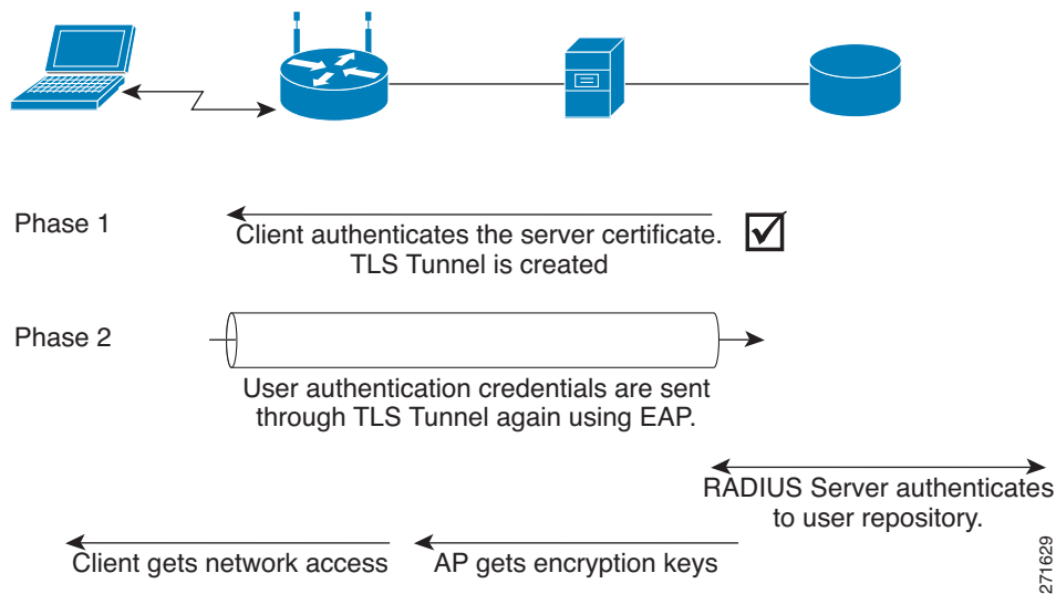
Figure B-3 PEAP Processing Flow
