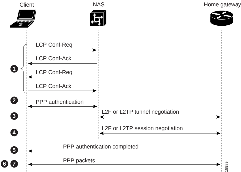
Figure 3 Protocol Negotiation Events Between Access VPN Devices
