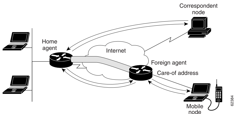
Figure 3 Reverse Tunnel
