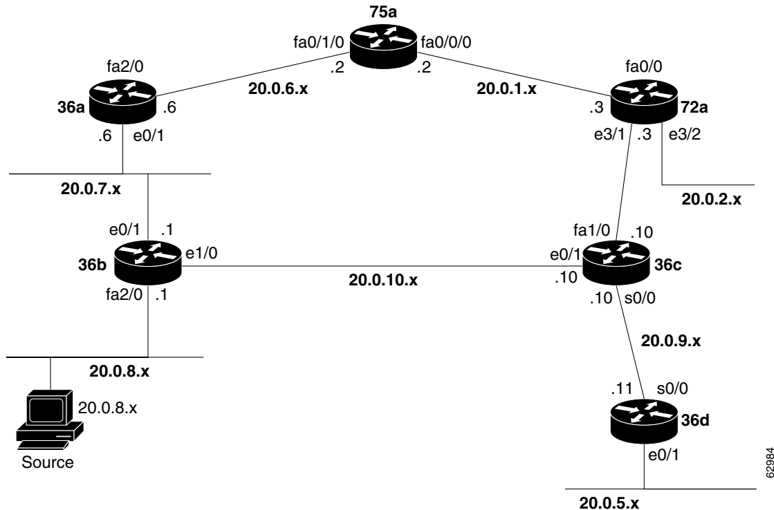
Figure 1 Network Topology Used for Sample Configurations
