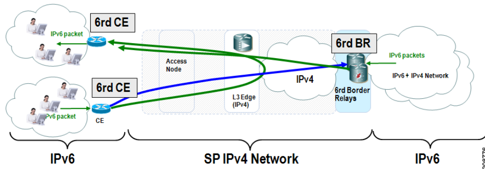
Figure 2 6RD Deployment
