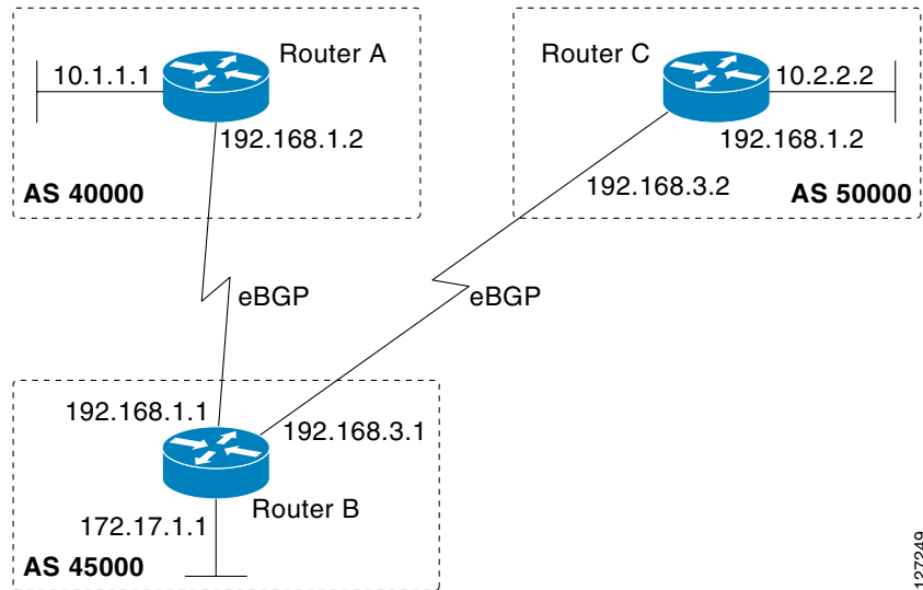
Figure 2 Multihoming Topology
