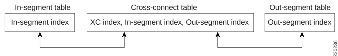
Figure 2 MPLS-LSR-STD-MIB Indexing
