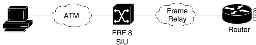
Figure 11 Frame Relay-to-ATM Interworking
