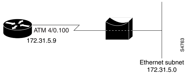
Figure 19 ATM Routed Bridge Encapsulation
