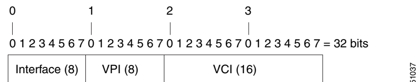
Figure 15 Format of the NAS-Port Attribute Field for PPP over ATM and PPPoE over ATM
