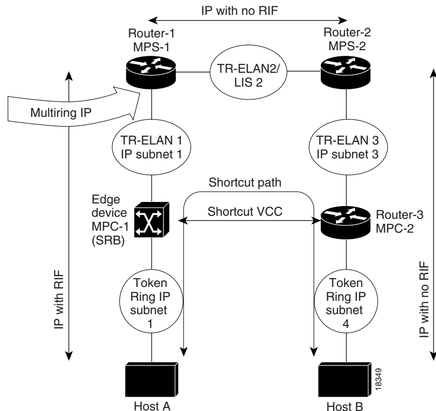
Figure 102 Token Ring MPOA—MPC to MPC Shortcut in an IP SRB-Routed Environment
