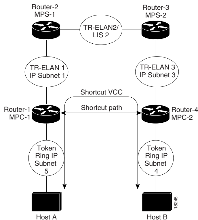
Figure 101 Token Ring MPOA—MPC to MPC Shortcut in an IP Routed Environment
