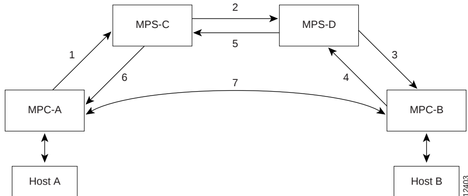
Figure 97 MPOA Message Flow Between MPCs and MPSs
