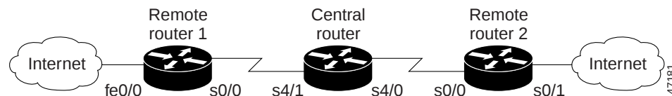
Figure 32 Sample Network Implementing DiffServ
