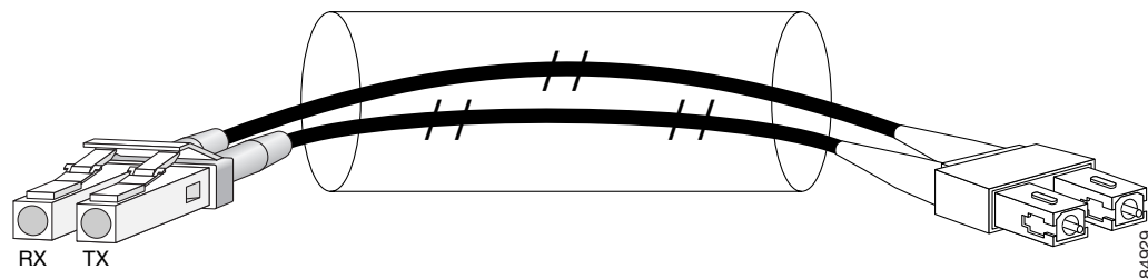
Figure 3-10 LC-Type Cable
